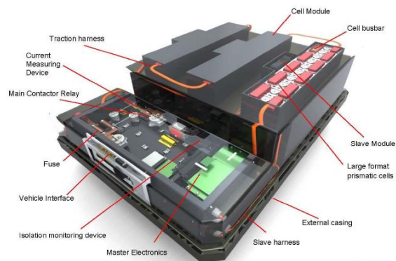
Fig. 7: Battery pack components [4]
