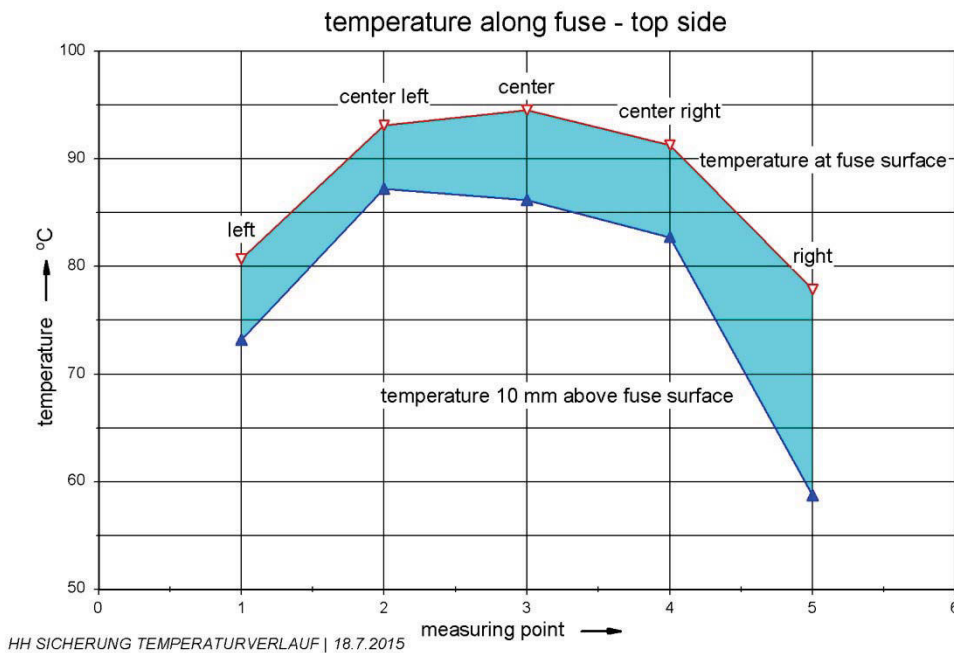
Fig 4: Difference of the temperature along fuse – top side, red curve: temperature at fuse, blue curve: temperature in the distance of 10 mm above the fuse
