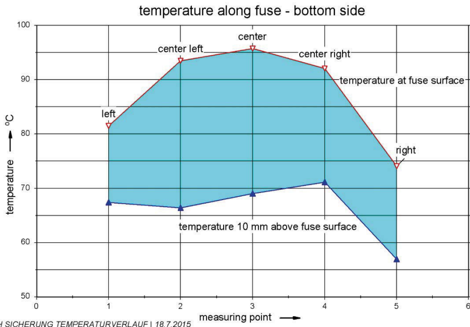
Fig 5: Difference of the temperature along fuse – bottom side, red curve: temperature at fuse, blue curve: temperature in the distance of 10 mm above the fuse
