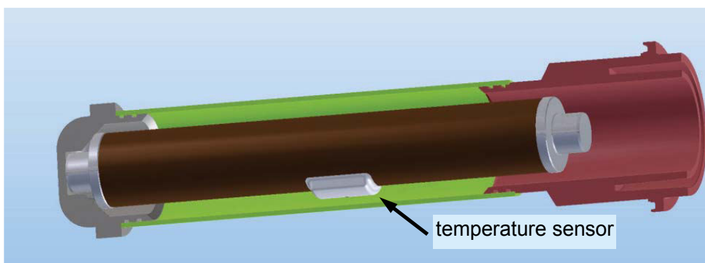
Fig. 6: Fuse with adapted temperature sensor
