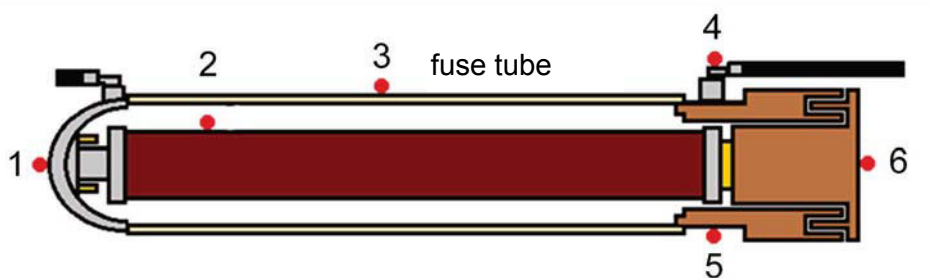
Fig. 2: Possible positions for thermal monitoring /5/
